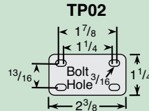
Swivel Plate
