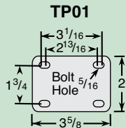
Swivel Plate
