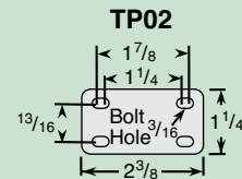
Swivel Plate
