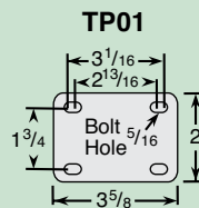
Swivel Plate
